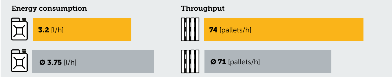
Consumption and transported pallets per hour according to VDI, compared to competition (average value)
